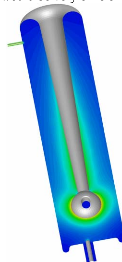
Figure 1: 88 MHz, \beta=0.07 cavity shape. Field shown is |E| at nominal coupling.
