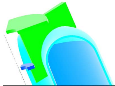
Figure 3: Strengthening structure for helium pressure frequency shift minimization.
