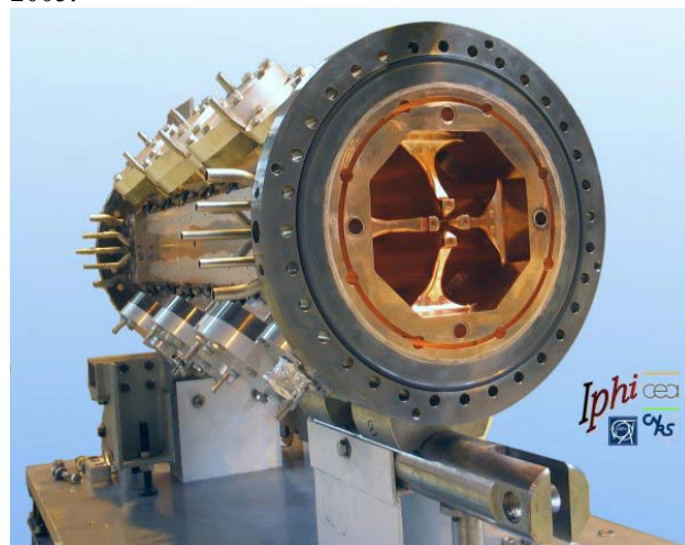
Figure 4 : the first RFQ section viewed from the beam entrance side.
