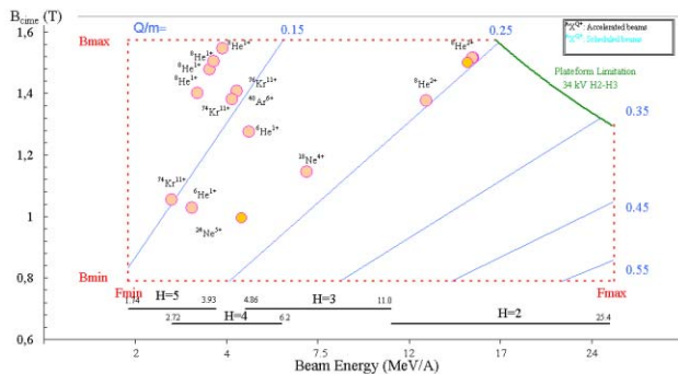
Figure 3 : CIME working diagram including accelerated beams (April 2004)
