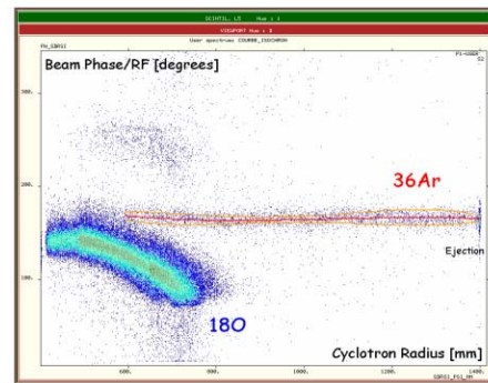
Figure 4 : Synchronism condition. Phase measurement as a function of the radius in CIME using a 300 \mu m silicon detector. Test realised on harmonic 3.
