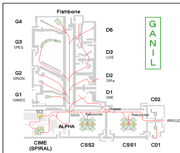
Figure 2: Plan of GANIL showing accelerators and experimental areas. C01 and C02 are compact cyclotrons ( E < 1 MeV.A); CSS1 ( E < 13.7 MeV.A) and CSS2 ( E < 95 MeV.A) separated sectors cyclotrons.
