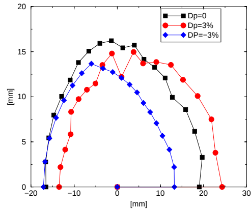
Figure 3: Dynamic Aperture.
