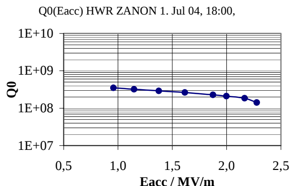
Figure 7: First Q_0 - E_{acc} measurement with low lHe-level
