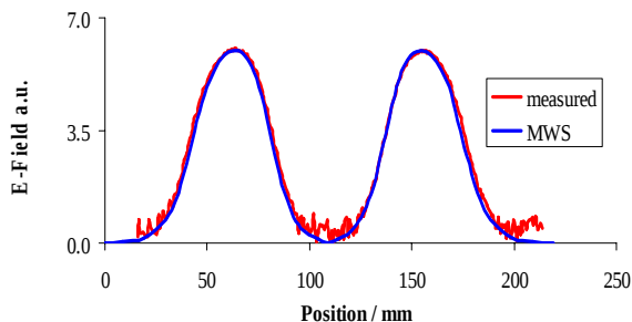
Figure 1: Field profiles: measured and calculated by MicrowaveStudio (MWS)
