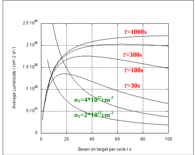
Fig. 2: Average luminosity for internal experiments with different beam lifetimes \tau (upper curves) assuming a target thickness of 2.5 \cdot 10^{15} \text{ cm}^{-2} , and for external experiments with a different target thickness n_T (lower curves) plotted versus beam on target time per cycle. 10^{11} circulating particles at 1MHz and a preparation time 7s were taken for this calculation.
