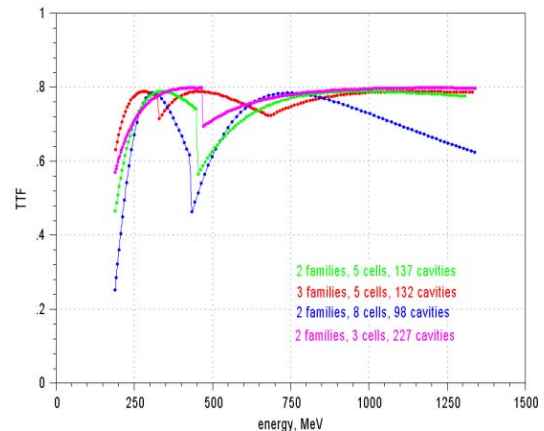
Fig. 2: Transient time factor of the ESS linac.
