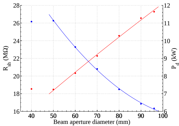
Figure 7: Drift-tube cavity - R_{sh} and P_d vs. beam aperture diameter.
