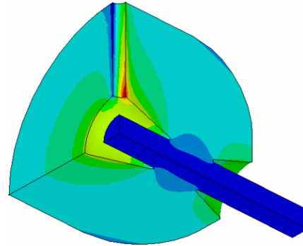
Figure 9: Magnetic field contour lines for the 50-mm beam-aperture drift-tube cavity.
