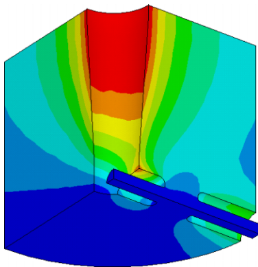
Figure 4: Magnetic field contour lines for the 50-mm beam-aperture half-wave resonator.
