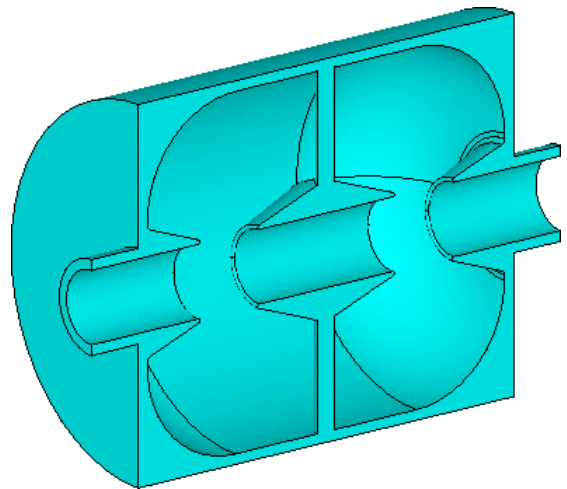
Figure 5: Cross section of the generic drift-tube cavity.
