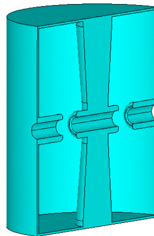
Figure 1: Cross section of the generic half-wave resonator.
