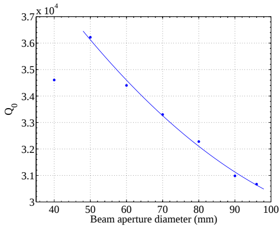
Figure 6: Drift-tube cavity - Q_0 vs. beam aperture diameter.
