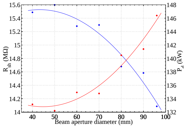
Figure 3: Half-wave resonator - R_{sh} and P_d vs. beam aperture diameter.
