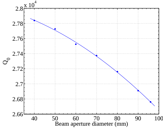
Figure 2: Half-wave resonator - Q_0 vs. beam aperture diameter.
