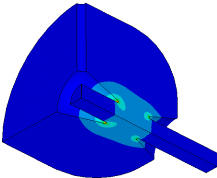
Figure 8: Electric field contour lines for the 50-mm beam-aperture drift-tube cavity.
