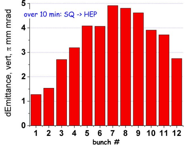
Fig.7: Emittance growth along pbar bunch train
