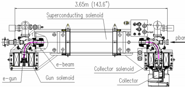
Figure 5: The first Tevatron Electron Lens.
