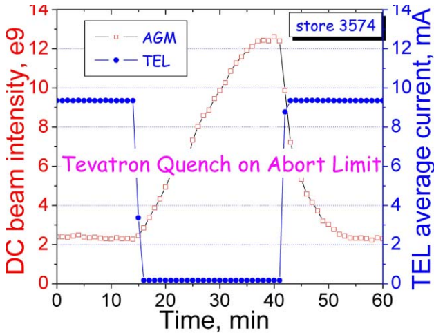
Fig.6: DC beam in abort gap with/without TEL
