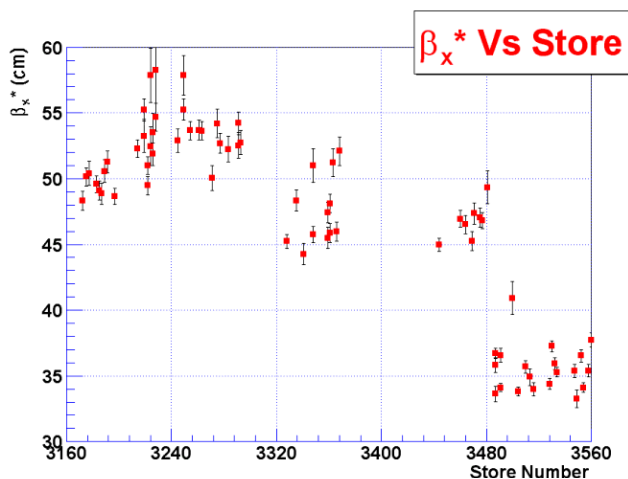
Fig.4: \beta^* as fit parameter of D0 luminous region analysis in stores from Jan., 13 to June 5, 2004, courtesy of J.Estrada, A.Chandra (D0 collaboration)
