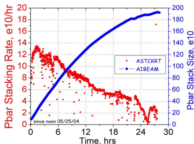
Fig.2: Typical cycle of Antiproton Accumulator operation
