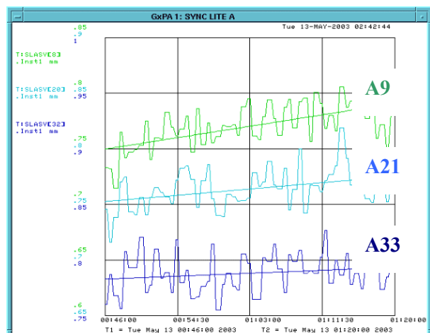
Fig.8: Vertical size of three pbar bunches in store 2540
