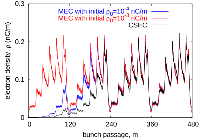
Figure 3: Electron cloud density evolution for bunch pattern (3,4,0)(6,8,0) using CSEC (black trace) and MEC with two different initial electron densities: \rho_0 = 10^{-4} nC/m (blue line) and \rho_0 = 10^{-3} nC/m (red line). No matter the initial electron density, both results agree for the last turn (from bunch passage 360 to 480).
