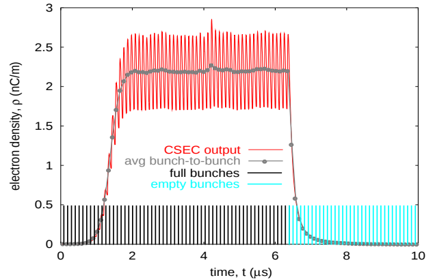
Figure 1: Time evolution of the electron density (red line) computed with CSEC during 10\mu s a (RHIC time revolution is 12.82\mu s ). The case corresponds to the injection of 60 successive bunches with a bunch spacing of 108 ns and a bunch intensity of N = 1.4 \times 10^{11} protons (marked with black bars), followed by 60 “empty” bunches (marked with light blue bars). The grey circles mark the average electron density between two consecutive bunches.
