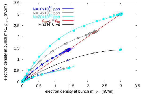
Figure 2: Average electron density after the bunch m passes by, \rho_{m+1} , as a function of the electron density before the bunch m passed by, \rho_m , for different bunch intensities, N . The lines correspond to cubic fits following Eq. 2.
