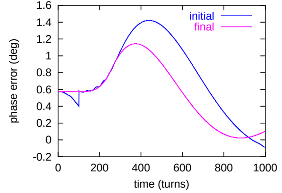
Figure 5: Phase error before and after optimization
