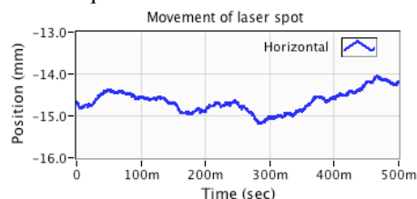
Figure 5. Horizontal position of laser spot over time.
