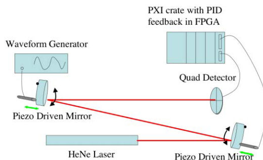
Figure 7. Setup to control drift.
