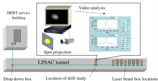
Figure 3. The setup of the laser drift measurement.
