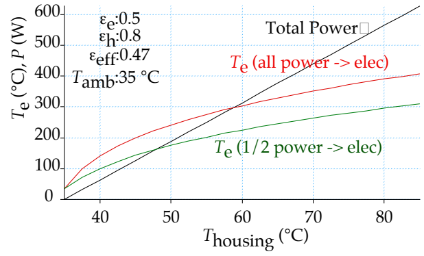
Figure 4: Electrode temperature.
