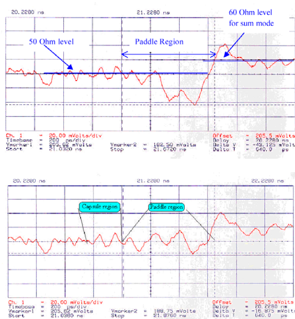
Figure 6: TDR with the old (top) and the new (bottom) paddles. Horiz. scale is 200 ps/div; vertical, 20 mV/div.
