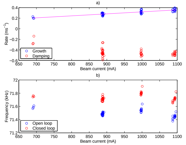
Figure 3: Transient measurements of horizontal EFEM -1 vs. beam current; a) Growth, damping rates, and a linear fit to growth rates; b) Growth (open loop) and damping (closed loop) modal oscillation frequencies
