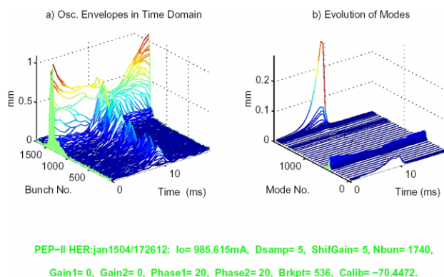
Figure 5: A vertical grow/damp transient showing significant motion of the bunches at the end of the train
