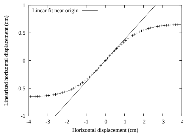
Figure 2: Linearized horizontal position measurement in an arc BPM. At a typical pretzel amplitude of 1.5 cm, the linearized formula shows significant disagreement with a linear fit.
