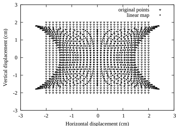
Figure 1: Distortion in CESR arc BPMs with approximately elliptical cross-section when linearization is used.
