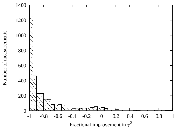
Figure 7: Fractional improvement in the \chi^2 of the beam position fit due to the calibration coefficients ( -1 = 100\% improvement).
