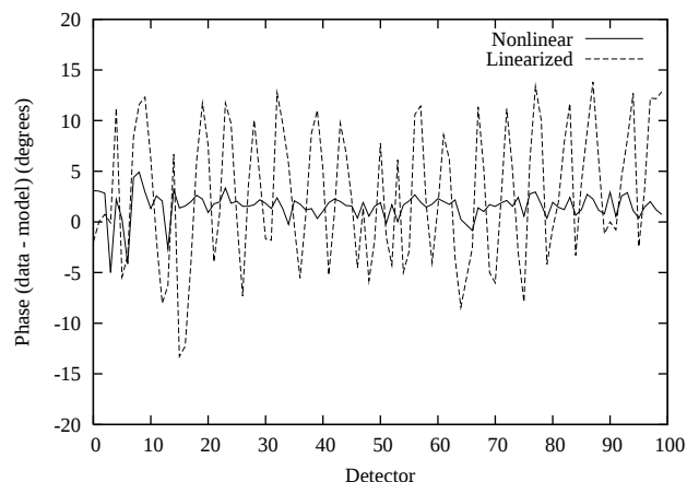
Figure 6: Difference in horizontal betatron phase advance between data and model with large closed orbit distortion after using a phase correction algorithm based on the linear (dashed) and nonlinear (solid) BPM evaluation.
