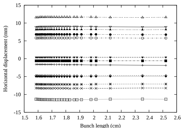
Figure 2: Beam position at various detectors showing little or no bunch length dependence.
