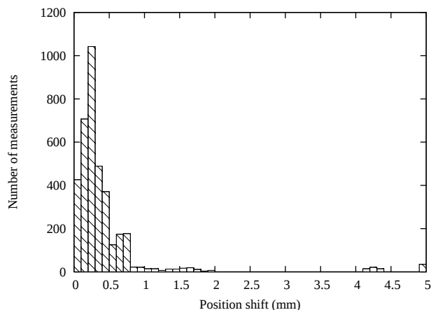
Figure 8: Correction in the calculated position due to the calibration coefficients.
