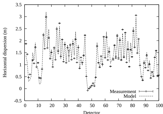
Figure 3: Measured and calculated dispersion.
