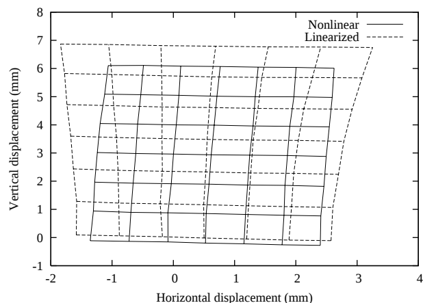
Figure 5: Separator scan. Orbits at detector 9W calculated using linearized (dashed) and nonlinear (solid) methods.
