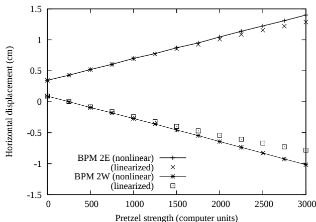
Figure 4: Beam position at two detectors calculated with the nonlinear and linearized methods.
