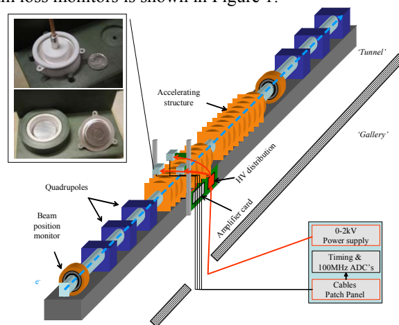
Figure 1: Layout of the beam loss system in a CTF3 linac module
