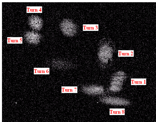
Figure 4: Superposition of pictures of the extracted beam after a variable number of turns before matching.
