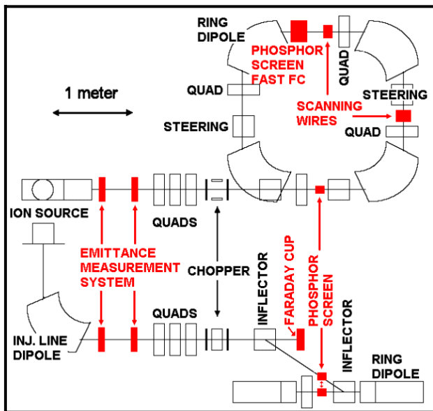
Figure 1: Top and side view of SIR. (Diagnostics in red)
