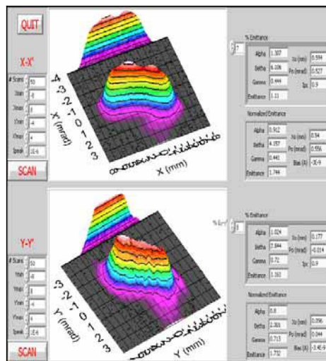
Figure 2: User interface of the emittance measurement system control program.
