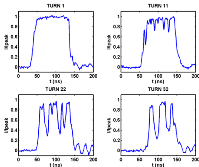
Figure 6: Longitudinal beam profiles measured with the Fast Faraday Cup when the beam is extracted after a variable number of turns.
