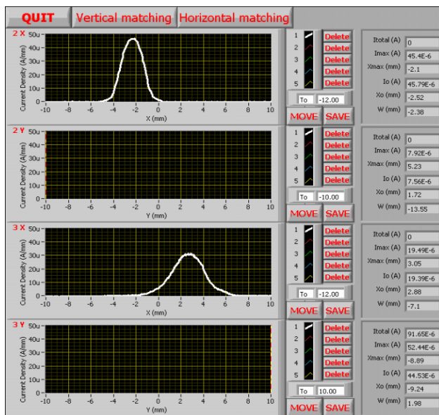
Figure 8: Front panel of the LabVIEW program used to move the two pairs of scanning wires.
