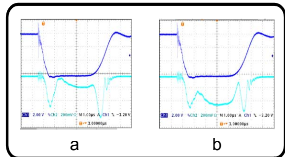
Figure 4. Accelerator reflected pulse
