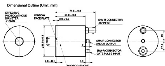
Figure 1. Hamamatsu gateable microchannel plate photomultiplier R5916U-50 Series.
