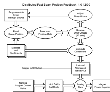
Figure 1: Flow diagram of the ALS fast feedback system. Timing of the system is completely network based, using a standard 100 MBit/s full duplex Ethernet which is also used for the data exchange between the 12 stations.
