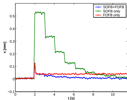
Figure 3: Response of the fast and slow orbit feedback systems to a step in a corrector magnet.
