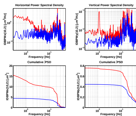
Figure 2: Power spectral density of the closed orbit motion between 0.1 and 50 Hz with the fast orbit feedback in open and closed loop. The measurements were taken with an independent acquisition system at a BPM not included in the feedback system. The noise floor is not subtracted in these plots.
