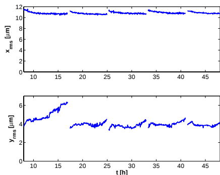
Figure 4: Rms orbit error over the course of 1.5 days. The first fill is after a beam dump, i.e. the thermal stability of the ring is not as good creating somewhat larger slow orbit drifts.
