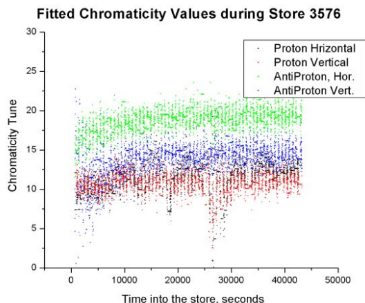
Figure 6: Proton and Antiproton chromaticities during the store.
