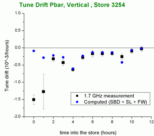
Figure 3: The antiproton tune drift during the store compared to expectation based on transverse and longitudinal emittance and intensity measurements
