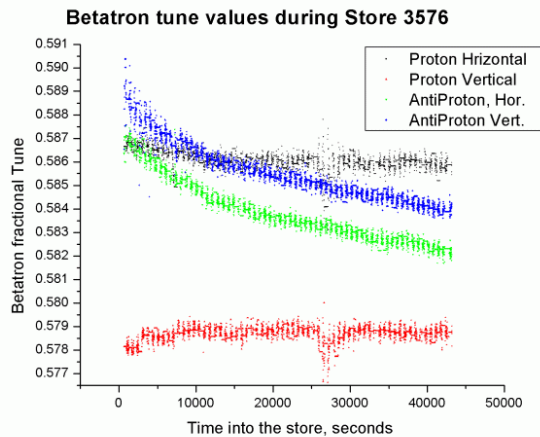
Figure 2: Proton and Antiproton fractional betatron tune during the store.
