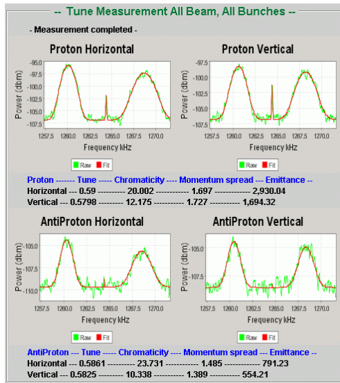
Figure 1: Online display of a randomly selected fit of the Schottky signals, for both proton and antiproton.
