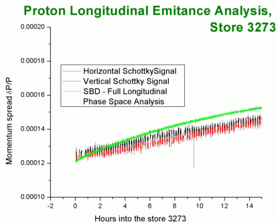
Figure 5: The momentum spread derived from the 1.7 GHz Schottky detector are consistent with those obtained from the Sample Bunch Display, which accurately measures the bunch length.
