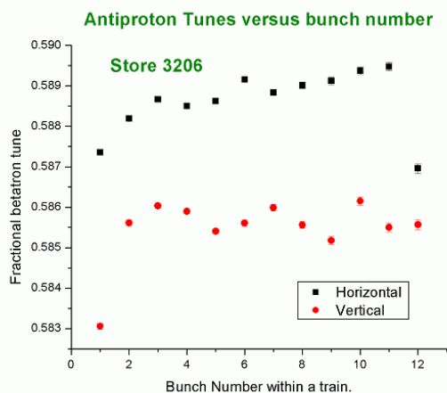
Figure 4: The antiproton tunes for all 12 bunches in the train, averaged over the three trains. The data was taken when tunes were fairly stable, staying only for a few minutes in a given gating configuration. The shift observed for the first and last bunches are significantly larger than our statistic or systematic accuracy.
