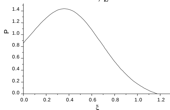
Figure 4. The universal profile of energy deposition.
