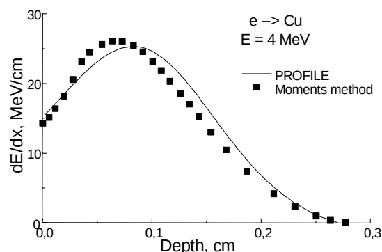
Figure 5. The energy deposition profile in Cu.
