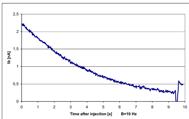
Figure 1: Current measurement with the Bergoz BCM. \text{H}_2\text{S}^+ ion beam current during 10 s with 66 averages.
