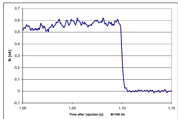
Figure 2: Current measurement made with capacitive pick-up. \text{D}^{13}\text{CO}^+ ion beam current with 4 averages. RF off after 1.1 s.
