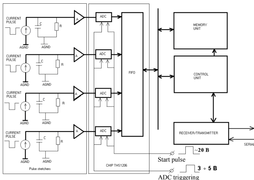
Figure 2: The electrical layout of the fast profile meter.
