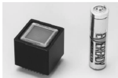
Figure 1: MAPMT R5900U-00-L16 HAMAMATSU
