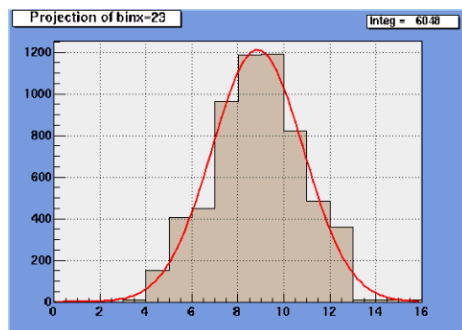
Figure 4: Example of the single beam profile fitted of the Gauss function.
