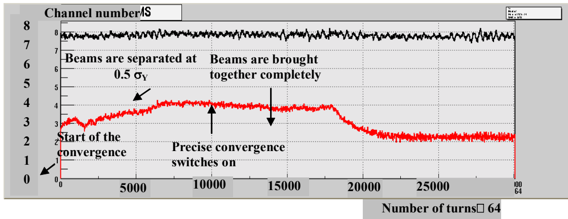
Figure 6: The position of center-of-weight of electron beam (upper line) and \sigma_Y behavior (down line) during the beams convergence in the interaction point. The total process duration is nearly 10^6 turns of the beams. Time of the single turn is 1220 ns. Channel constant is 0.2 mm.
