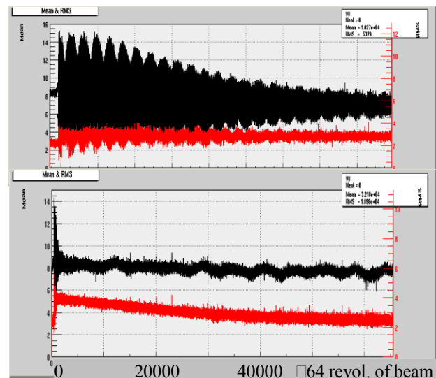
Figure 5: Beam profile dynamic after kick. Upper curve of every plot is a centre-of-weight of the beam. Down curve represents behavior of the beam size \sigma_Y .
