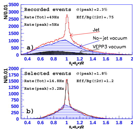
Figure 2: The distributions over parameter R for typical 1 hour run. a) no selection; b) background suppressed.
