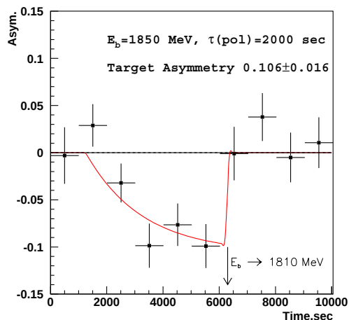
Figure 4: Measurement of the asymmetry in the processes of build-up of the polarization and crossing spin resonances.
