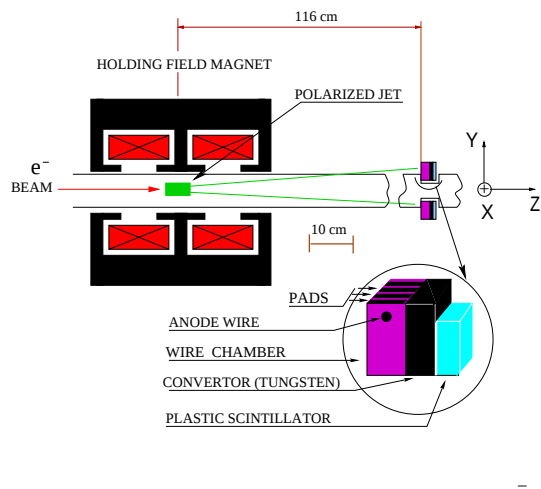
Figure 1: Lay-out of Møller Polarimeter with Internal Target.
