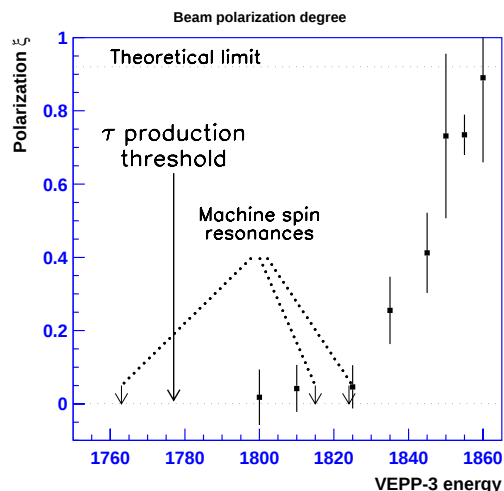
Figure 3: Measured Beam Polarization degree vs. VEPP-3 Beam Energy
