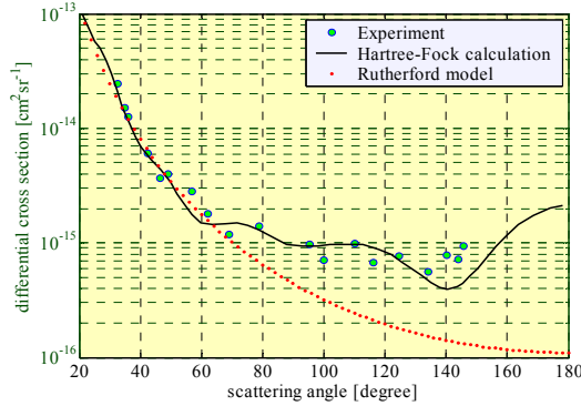
Figure 4: Differential cross section for the elastic electron scattering from \text{Xe}^{+6} ions[2].
