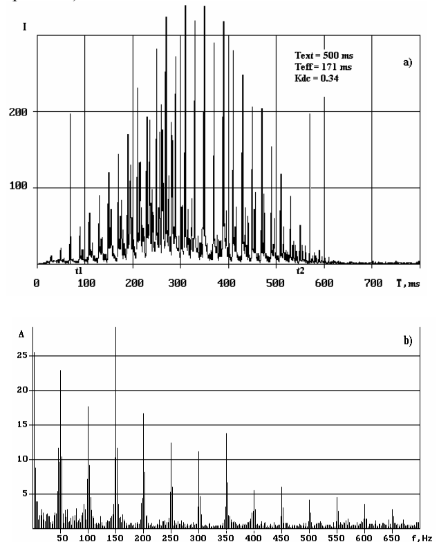
Figure 4: Beam spill characteristics without an active filter of LQ and without feedback.
