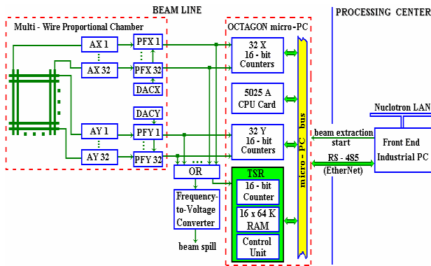
Figure 3: Block-diagram of the digital-mode MWPC electronics.
