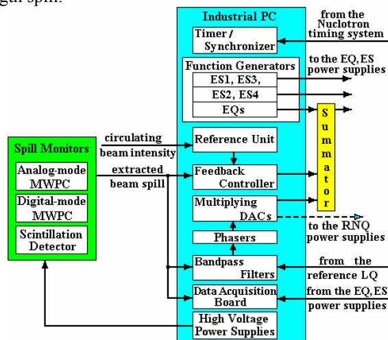
Figure 5: Schematic diagram of the spill control subsystem.
