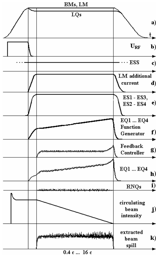
Figure 2: Timing chart of extraction processes.
