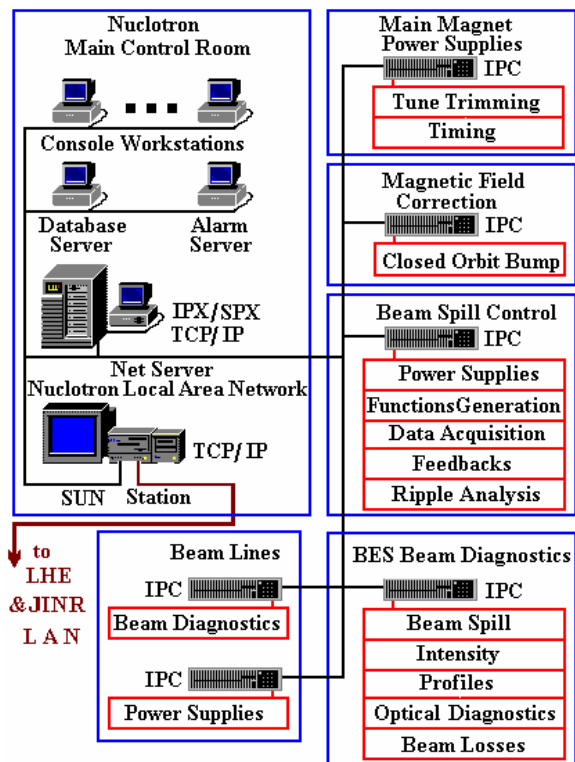
Figure 1: BES control subsystem structure.
