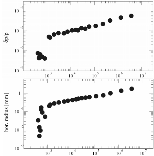
Fig.1. Beam behavior in the ESR experiment showing the anomalous temperature reduction at low intensity. Momentum spread and beam size are given as functions of number of stored ions. ^{238}\text{U}^{92+} 400 MeV/u
