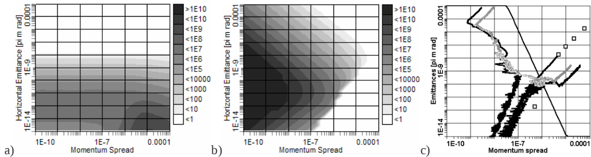
Fig.2. The theoretical dependence IBS growth rates on beam emittance and momentum spread for ESR: a) – horizontal component of IBS growth rates, b) – longitudinal one. Results of MD calculations (c): evolution of ion beam parameters during the cooling, solid black line corresponds to cooling rate 4 \cdot 10^4 Hz, grey circles – 10^4 Hz, straight line is criterion \Gamma_2 = \pi ( N = 5 \cdot 10^5 ). Square points – ESR experiment (Fig.1).
