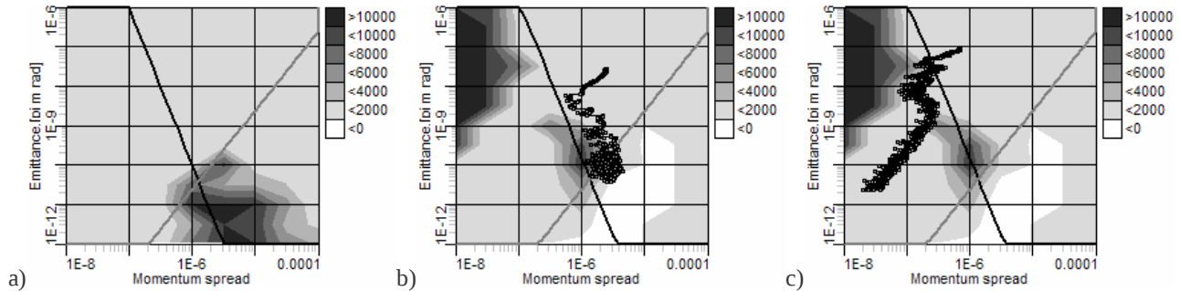
Fig.3. MD simulation: a)- horizontal component of IBS growth rates, b), c) - longitudinal component of IBS and evolution of beam parameters during cooling process. I_{cool} = 5 A, ^{132}\text{Sn}^{50+} 220 MeV/u, N = 10^5 .
