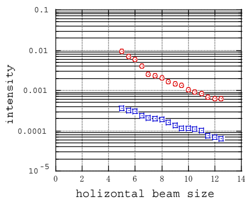
Fig. 8 Comparison of beam tails; circles denote beam tail without opaque disk, ;squares denote beam tail measured with opaque disk and Lyot stop. The horizontal axis is normalized by 1\sigma of the beam size.
