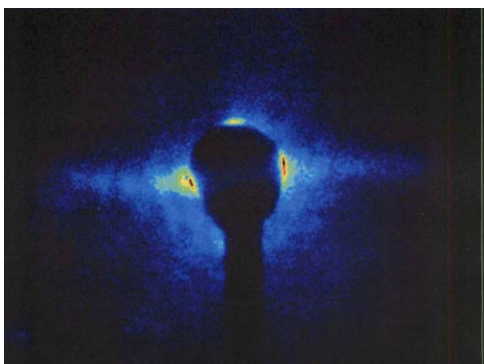
Fig.7 Image of beam tail with the opaque disk. Transverse magnification is same as in Fig.6. Exposure time of CCD camera is 10msec.
