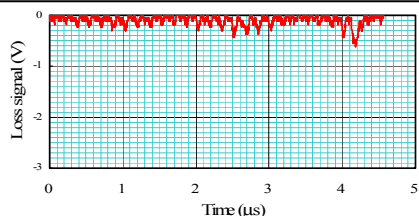
Figure 7: Best trigger timing of kicker magnet
