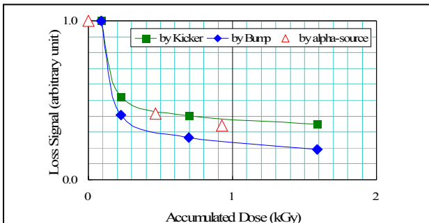
Figure 11: Decrease of signal in scintillation fiber by accumulated Dose (Beam loss is generated by firing kicker and bump magnet, respectively.)
