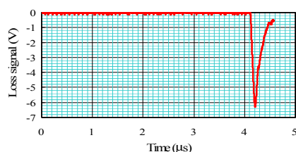
Figure 6: Bunched beam loss due to kicker field
