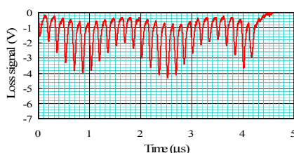
Figure 5: Bunched beam loss due to bump field
