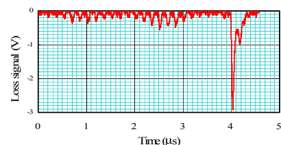
Figure 8: Beam loss due to bad trigger timing of kicker magnet 30ns earlier than the best
