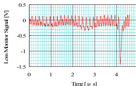
Figure 9: Pulse signal generated in the scintillation fiber caused by the beam going through 500MeV-BT
