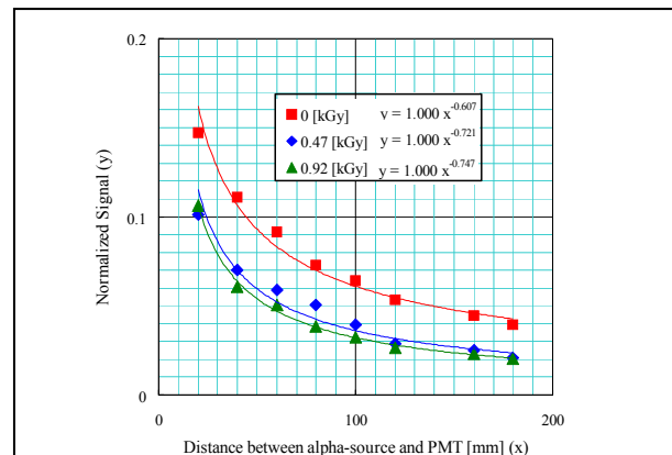
Figure 14: Normalized signal dependence in the scintillation fiber on the position of \alpha -source
