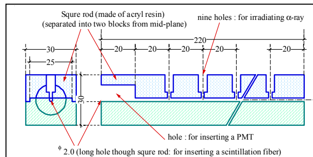
Figure 13: Sample holder to measure the dependence of the signal on the position of \alpha -source
