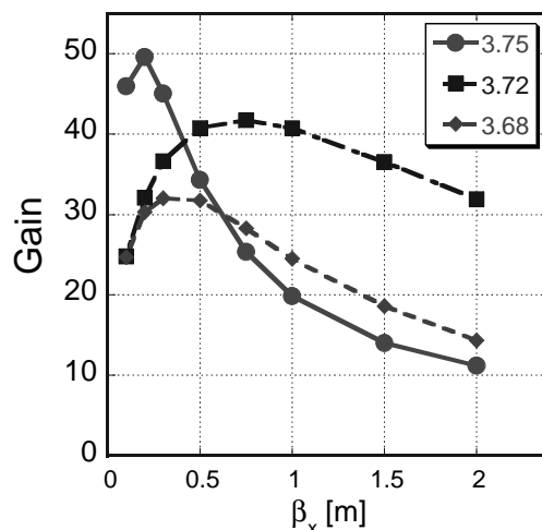
Fig. 1: The multiturn-injection gain as a function of beta function of the injection beam at three different horizontal-tune values.
