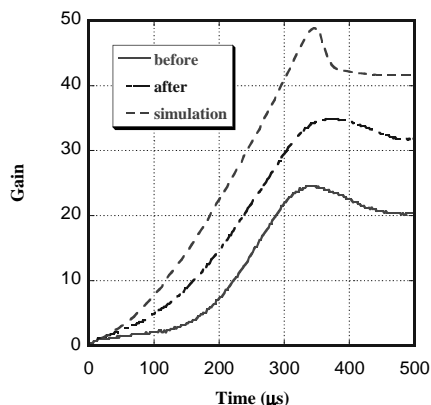
Fig. 6: The injection gain during the multiturn injection and 150 \mu s after the end of the injection.
