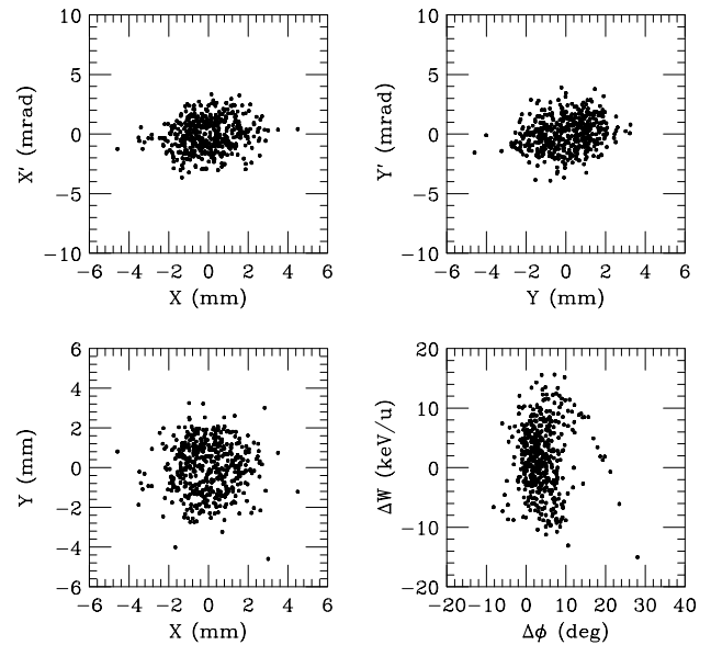
Fig. 5: The phase space and X-Y distribution for the extracted beam from the IH-DTL.
