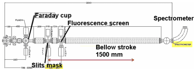
Figure 2: Emittance-meter design.
