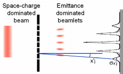
Figure 1: Multi-slits mask intercepting a space charge dominated beam.
