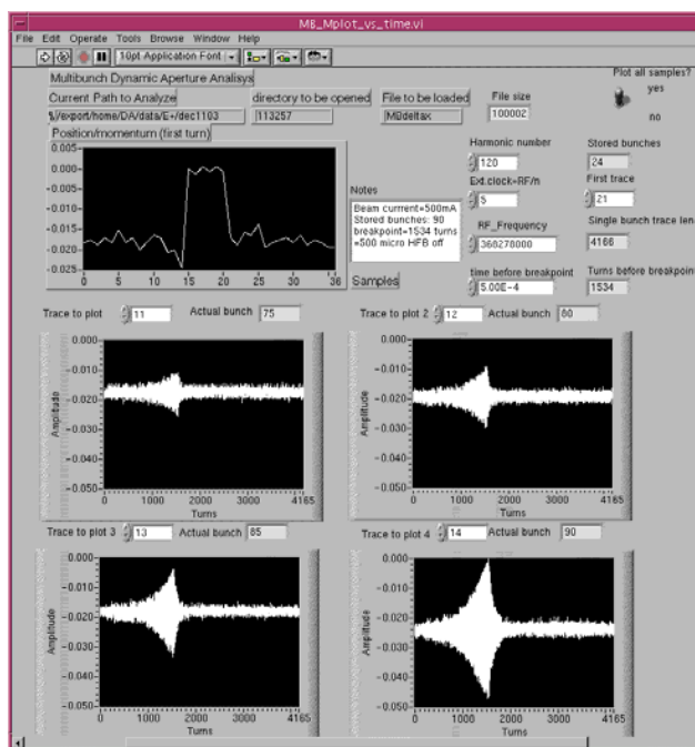
Figure 2 – Hor.instability grow/damp for the bunches 75, 80, 85, 90 versus revolution turns (1 turn = 324 nsec)
