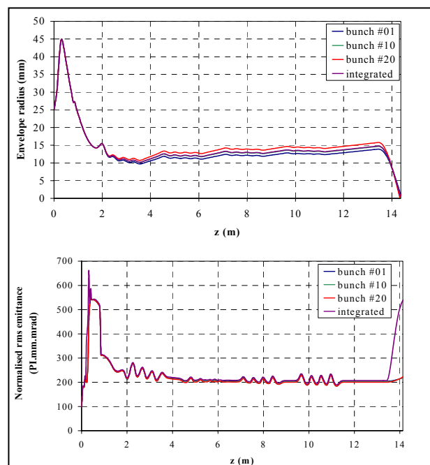
Figure 6: Evolution of beam ( first, middle and last bunch, full pulse) parameters along the accelerator. UP: Envelope radius, DOWN: rms normalised emittance.
