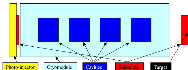
Figure 1: Accelerator schematic layout.
