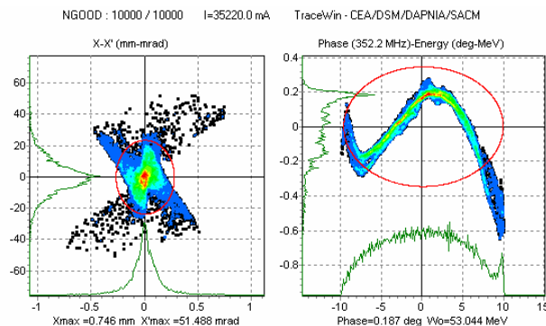
Figure 5: First bunch transverse and longitudinal phase-space distribution on the target.
