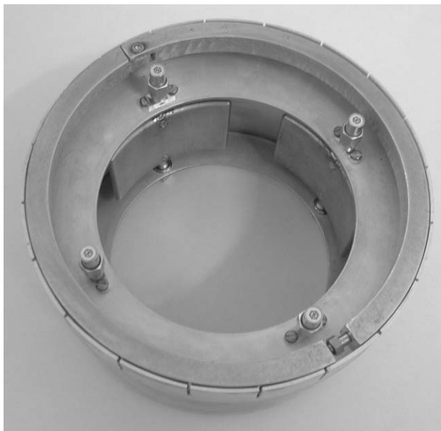
Figure 1: The beam position monitor.
