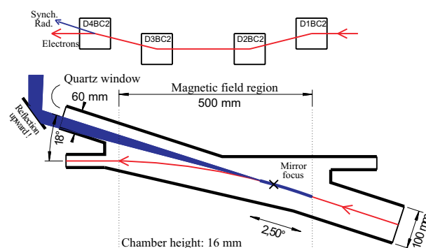
Figure 2: BC2 layout and D4BC2 vacuum chamber.
