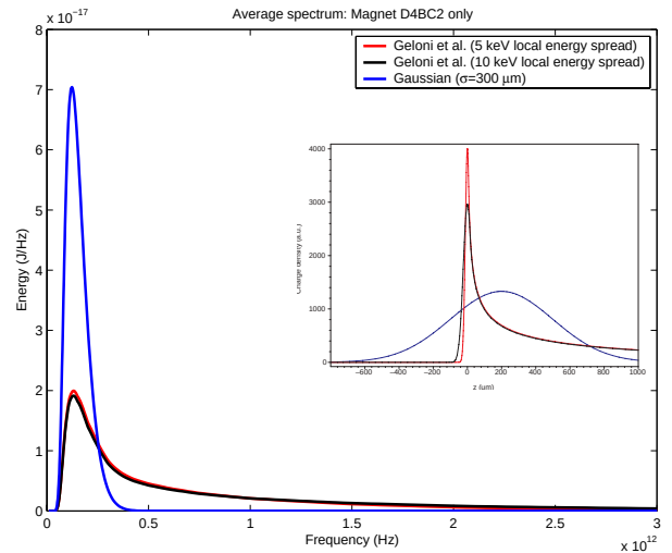
Figure 5: Simulated spectrum including form factor for the bunch shapes shown in the inset, chamber cut-off and window transmission.
