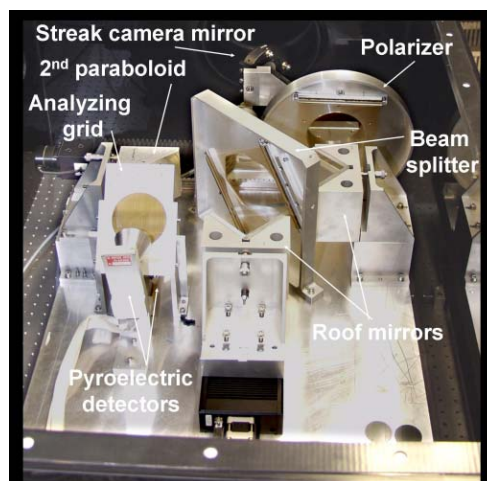
Figure 3: The Martin-Puplett interferometer.
