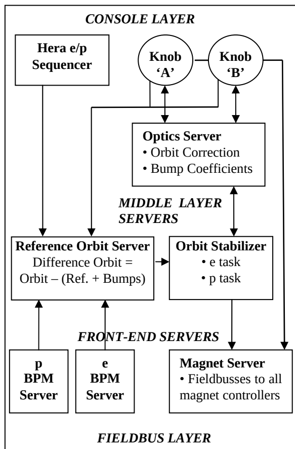
Figure 1: Communications for the orbit stabilization.
