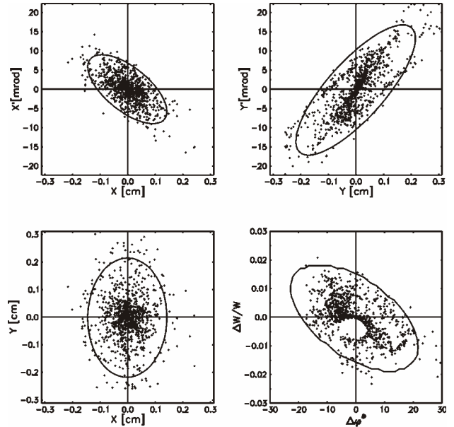
Figure 8: Particle distribution at the End of the RFQ-electrodes.
