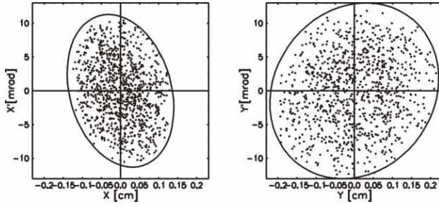
Figure 6: Distribution of fig. 5 transformed to the position of the electrodes entrance.
