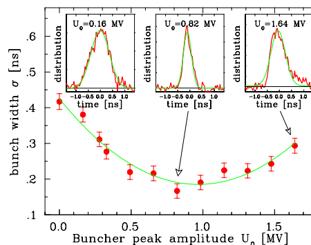
Figure 3: Measurement of the bunch width (one standard deviation) as a function of the buncher voltage 31 m upstream to the detector performed with a 2 mA \text{Ni}^{14+} beam.
