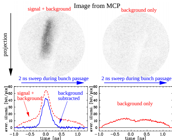
Figure 2: Typical image (inverted color) from the MCP for a 60 \mu\text{A Au}^{25+} beam averaged over 16 macro-pulses with 1 ms duration and a vacuum pressure of 6 \cdot 10^{-5} mbar. 8 W had been fed to the 108 MHz rf-deflector. The background is displayed right.
