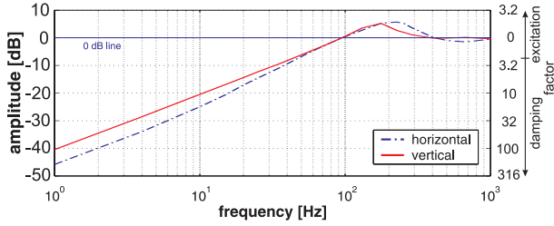
Figure 1: Measurement of FOFB closed loop transfer functions in both transverse planes. Effective damping of orbit perturbations has been achieved close to the FOFB design goal of 100 Hz.
