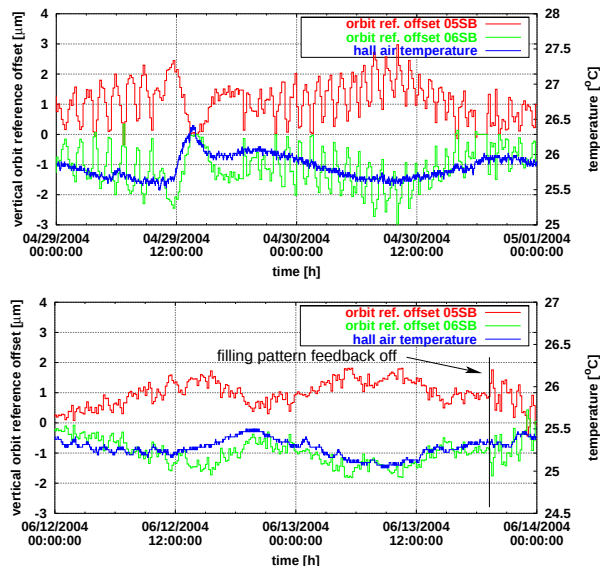
Figure 3: FOFB reference orbit changes of the two RF BPMs (05SB, 06SB) adjacent to the ID. An asymmetric bump is applied by a high level slow feedback in order to keep the photon BPM reading constant. With the filling pattern feedback a 40-50 minute oscillation (upper plot) due to a filling pattern dependence of the BPM system could be eliminated (lower plot). The remaining drift is mainly due to air temperature variations at the location of the BPM electronics.
