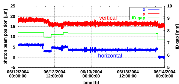
Figure 4: Resulting photon beam position at the X06S protein crystallography (PX) beamline over a period of two days with an active slow high level feedback on top of the FOFB to stabilize the position. The readings have been averaged over a period of 1s. A gap change results in a new reference position for the high level PBPM feedback.
