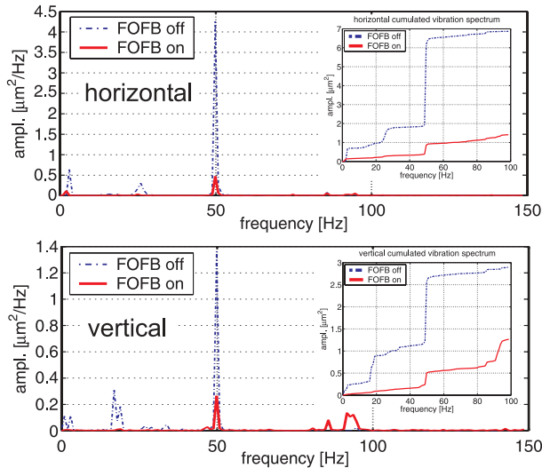
Figure 2: Snapshots of the horizontal and vertical power spectral densities measured at the tune BPM outside the orbit feedback loop. The cumulated power spectral density is shown in the small embedded plots on the right hand side.
