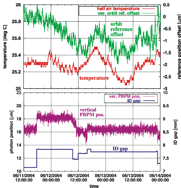
Figure 4: A slow PBPM feedback changes the electron beam reference position (top) of the two adjacent BPMs to ID X06S (only ARIDI-BPM-06SB is shown) in order to keep the photon beam stable to a sub- \mu\text{m} level (bottom) at the PBPM monitor. The applied asymmetric bump mainly compensates a systematic temperature dependency of the DBPM electronics. Each ID gap change leads to a new reference position for the PBPM feedback.
