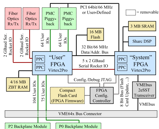
Figure 1: Simplified Block Diagram of the VPC Board
