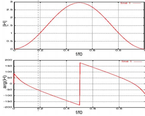
Figure 4: Example of FIR filter used for the transverse feedback. Design phase is -50 degrees at betatron tune of 0.18 (marked by dashed line). The frequency is normalized to the revolution frequency f_0 .
