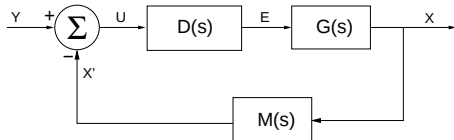
Figure 2: Basic Feedback Loop. G(s) denote the plant's, M(s) the monitor's and D(s) the controller's transfer function. X is the actual, X' the measured and Y the reference state of the plant that is driven by the excitation signal E .
