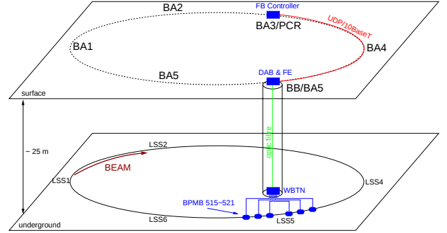
Figure 1: Site map of the orbit feedback components that are used for the SPS studies. The BPMBs and CODs are installed in LSS5, while the feedback control is performed in PCR.
