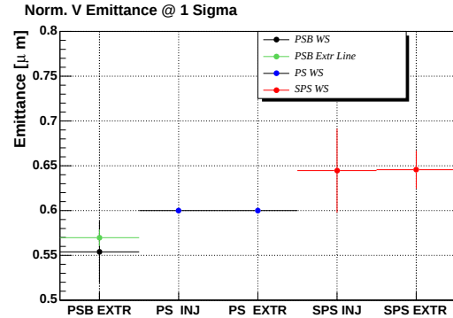
Figure 6: Vertical emittance evolution of the "pilot" bunch in the LHC pre-accelerators.
