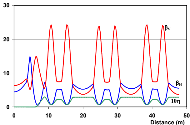
Figure 3: The Double Bend with a 7.0 m zero dispersion straight. One quarter of the lattice is shown.
