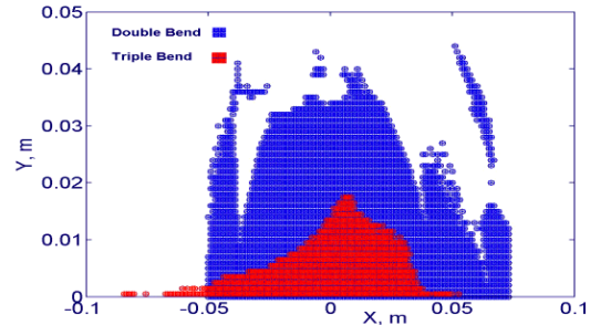
Figure 6: Tracking over 1000 turns for both lattices.
