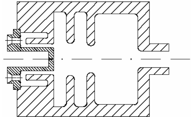
Fig. 1: Cross section of the gun.
