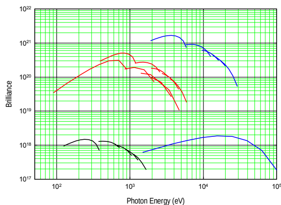
Fig. 2. Brilliance curves for the MAX IV rings.
