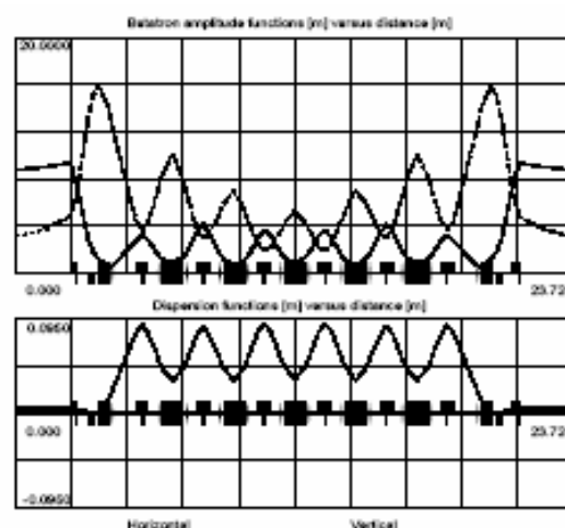
Figure 1: Machine functions for the MAX IV rings.
